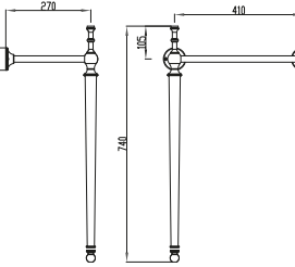
HARROGATE SMALL BASIN FRAME
