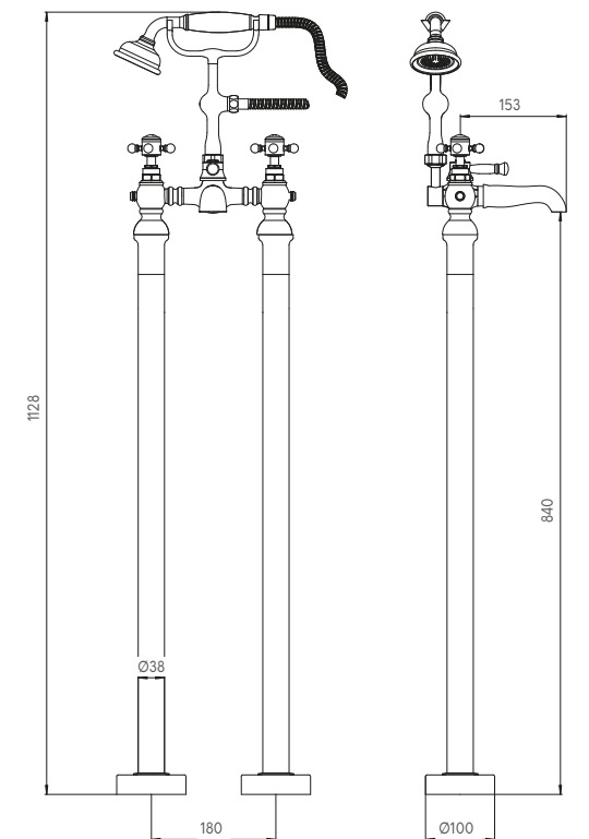
FREESTANDING BATH SHOWER MIXER
