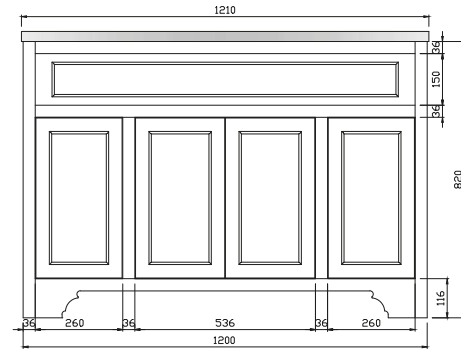
DUCHY 1200 VANITY UNIT
