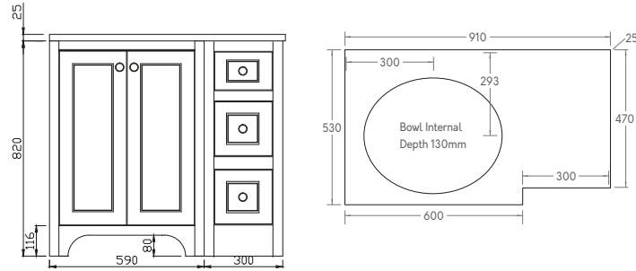
BRUNSWICK 900 RETURN UNIT LEFT
