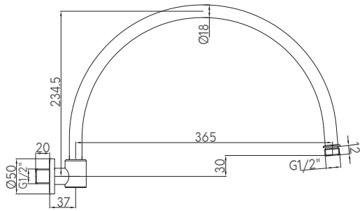
TRADITIONAL WALL ARM
