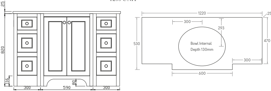
BRUNSWICK 1200 UNIT
