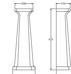
HARROGATE PEDESTAL
