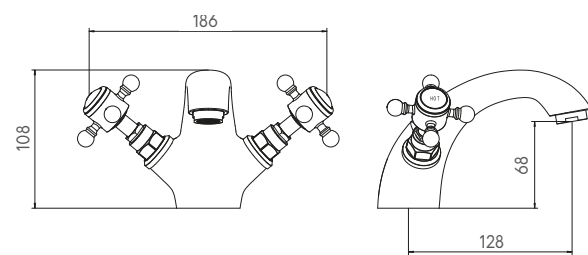
MONO BASIN MIXER WITH PUSH WASTE
