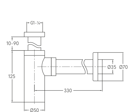
BOTTLE TRAP
