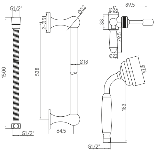
TRADITIONAL RIGID RISER KIT
