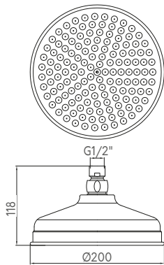
TRADITIONAL RAINCAN SHOWER HEAD
