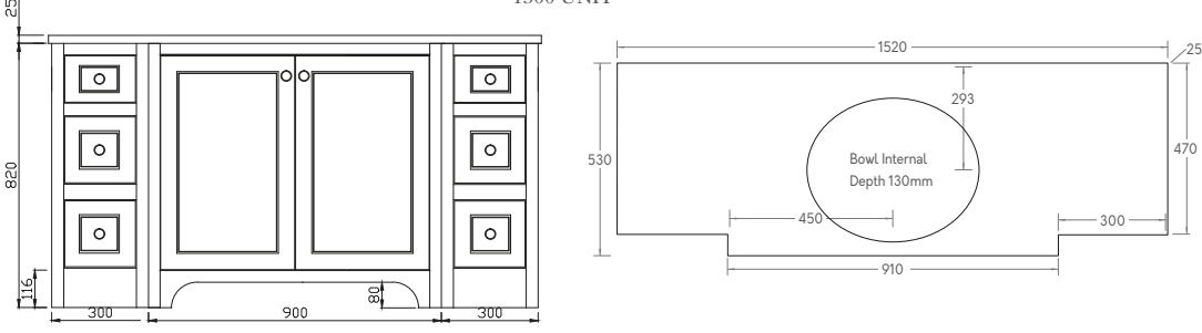
BRUNSWICK 1500 UNIT
