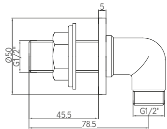
TRADITIONAL OUTLET ELBOW
