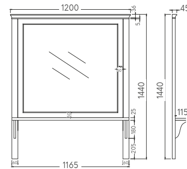
HARROGATE WALL MIRROR 1200 x 1400MM
