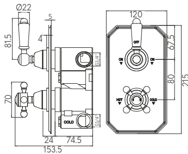
TRADITIONAL CONCEALED VALVE WITH DIVERTER
