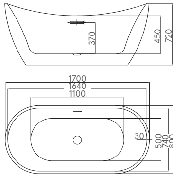
ARUBA ACRYLIC FREESTANDING BATH
