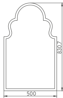
HARROGATE AGED BRASS/CHROME MIRROR
