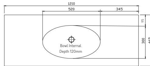
SINGLE BASIN
