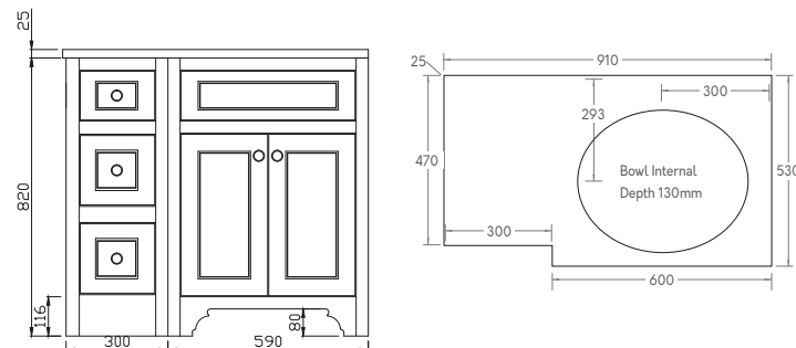
RIPLEY 900 RETURN UNIT RIGHT
