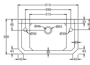
HARROGATE SMALL BASIN
