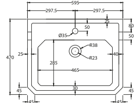
HARROGATE LARGE BASIN
