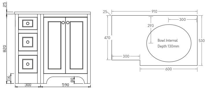
BRUNSWICK 900 RETURN UNIT RIGHT
