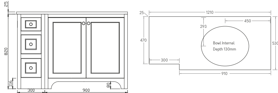
BRUNSWICK 1200 RETURN UNIT RIGHT
