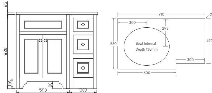
RIPLEY 900 RETURN UNIT LEFT
