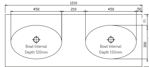
TWIN BASIN
