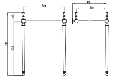
HARROGATE LARGE BASIN FRAME
