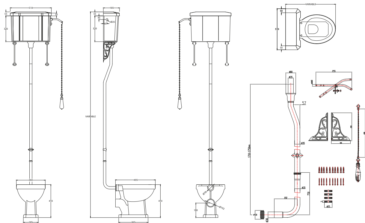
HARROGATE HIGH LEVEL WC
