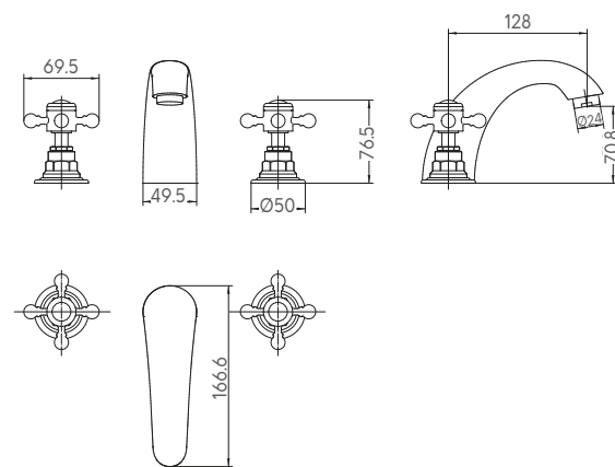
3 HOLE BASIN MIXER
