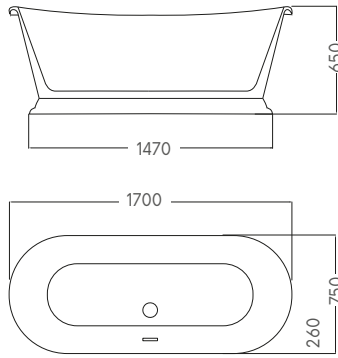
MAYFLOWER ACRYLIC FREESTANDING BATH
