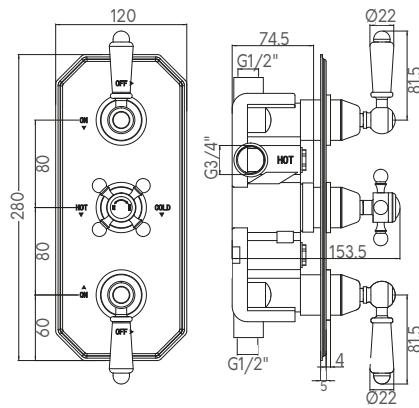
TRIPLE TRADITIONAL CONCEALED VALVE
