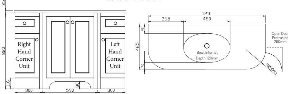
BRUNSWICK CURVED 1200 UNIT
