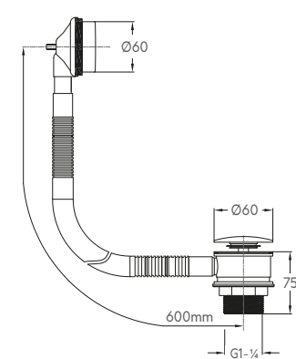
BATH POP-UP WASTE WITH OVERFLOW
