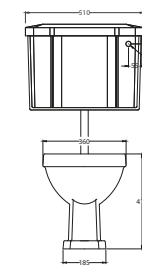
HARROGATE BACK TO WALL PAN
