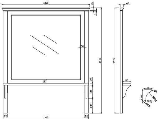
HARROGATE 1200 x 1400 WALL MIRROR
