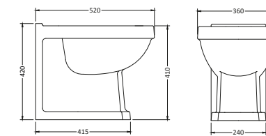
HARROGATE BACK TO WALL PAN
