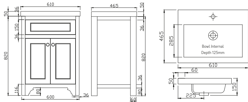
RIPLEY 600 VANITY UNIT
