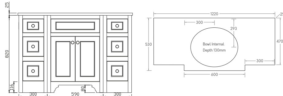
RIPLEY 1200 UNIT
