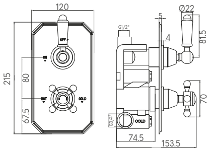
TRADITIONAL CONCEALED VALVE
