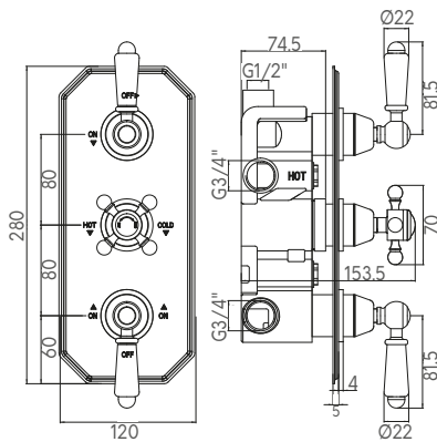
TRIPLE TRADITIONAL CONCEALED VALVE WITH DIVERTER
