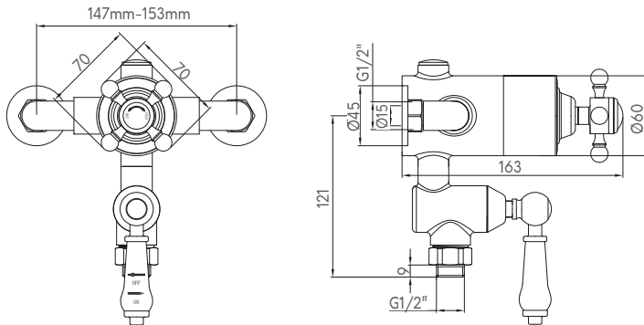
TRADITIONAL EXPOSED VALVE
