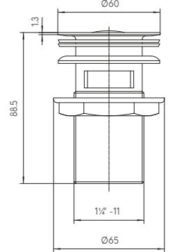
SPRUNG BASIN WASTE
