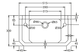
HARROGATE WALL HUNG BASIN
