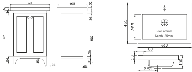
BRUNSWICK 600 VANITY UNIT
