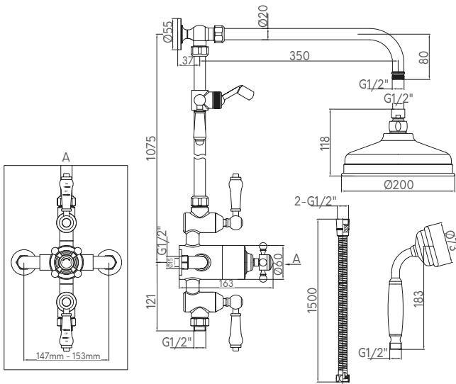
TRADITIONAL RIGID RISER SHOWER
