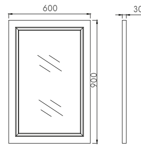
HARROGATE WALL MIRROR 600 X 900MM
