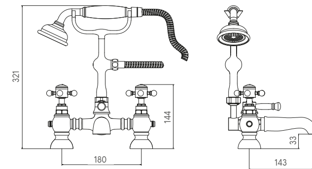
BATH SHOWER MIXER WITH CRADLE
