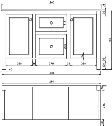
MONTPELIER 1200 VANITY UNIT
