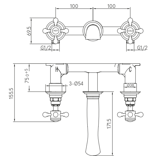
WALL MOUNTED BASIN MIXER
