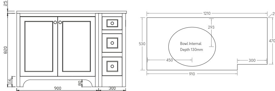
BRUNSWICK 1200 RETURN UNIT LEFT
